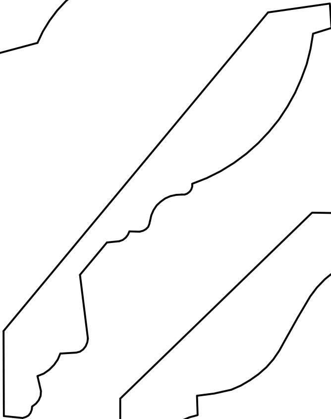
CR-1008 SIZE 3/4" THICK X 5 3/8" WIDE PROJECTION 3 11/32" DROP 4 7/32"
