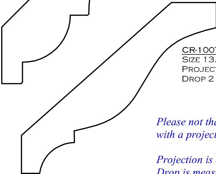
CR-1005 SIZE 7/8" THICK X 4 1/2" WIDE PROJECTION 3 3/16" DROP 3 1/8"
