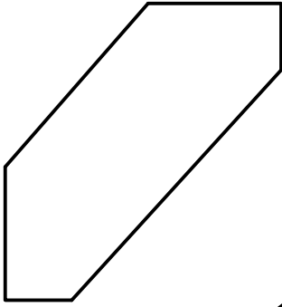
CR-1009 SIZE 3/4" THICK X 2 9/32" WIDE PROJECTION 1 9/16" DROP 1 21/32"
