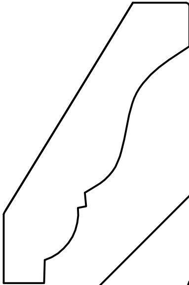
CR-1004 SIZE 3/4" THICK X 3 1/2" WIDE PROJECTION 1 15/16" DROP 2 7/8"
